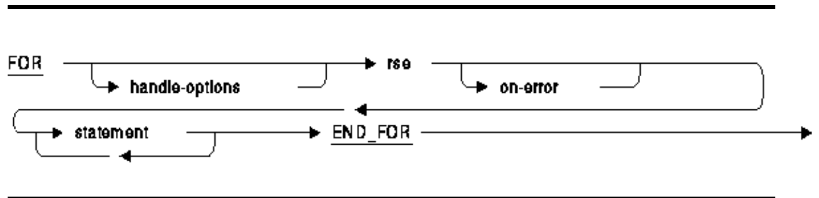
Example 5–3 FOR Format
